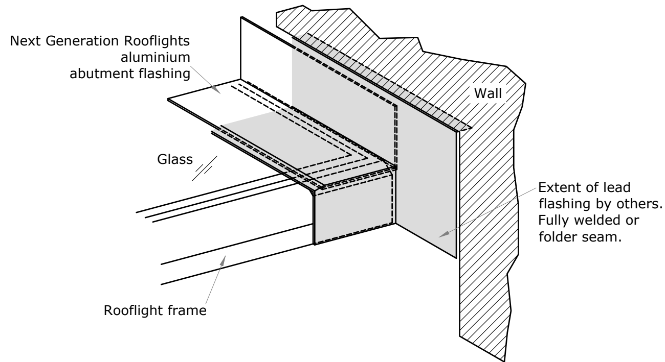
Isometric view of lead weathering requirements (NTS)
